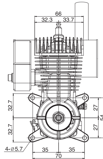
Dimensions (mm)
